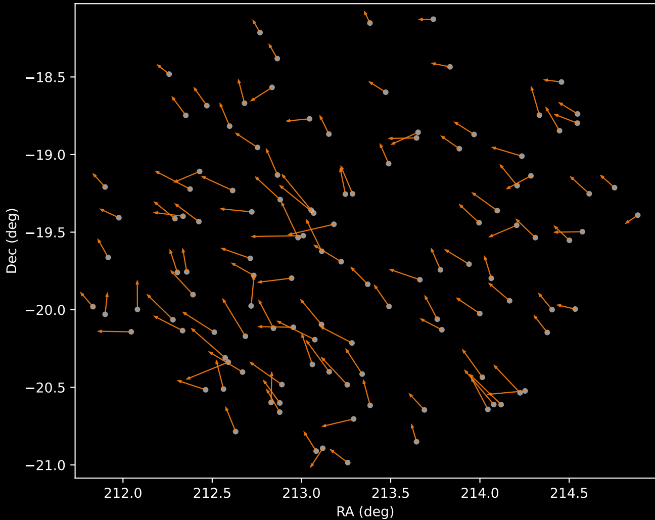
APOGEE DR17 Cluster 2 Proper Motion Vectors (n=118)
