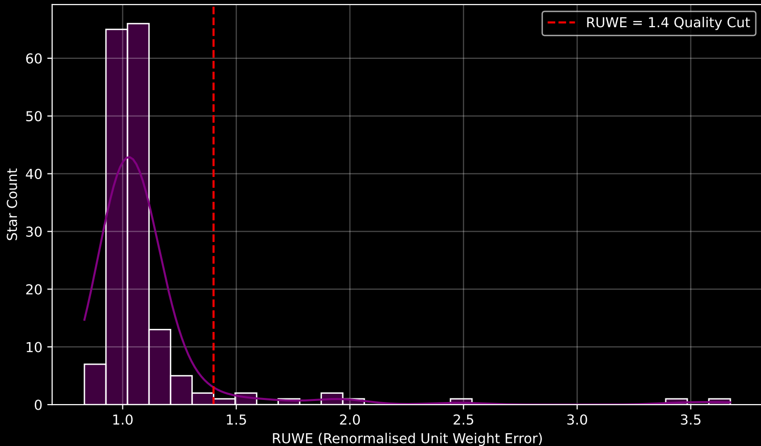
GAPOGEE DR17 Field [235+00] RUWE Distribution (n= 168)
