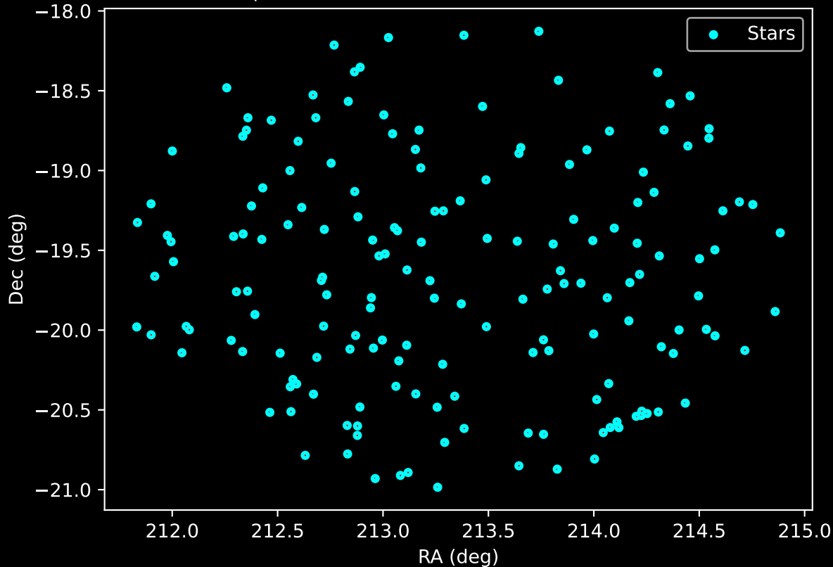
APOGEE DR17 Field: [235+00] Proper Motion Vectors for Gaia Star Field (n= 170)
