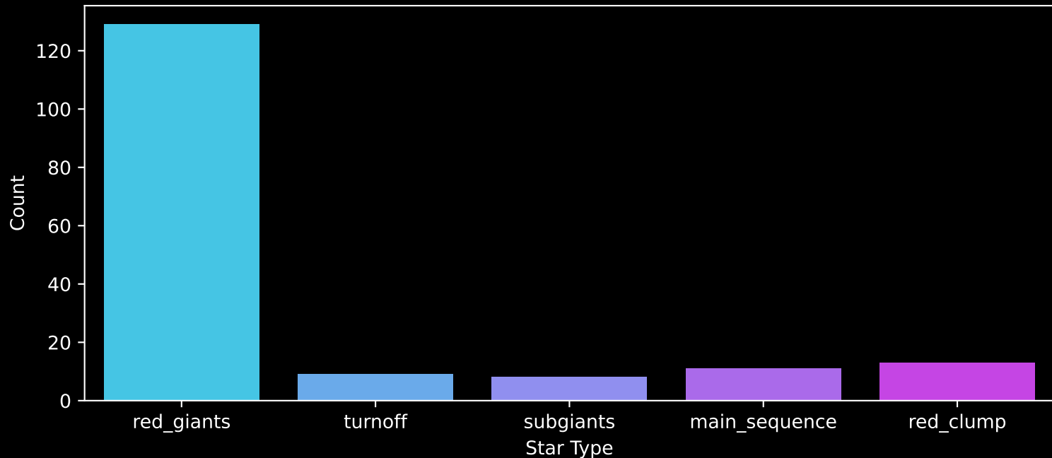
APOGEE DR17 Field: [235+00] Count plot of Star Type
