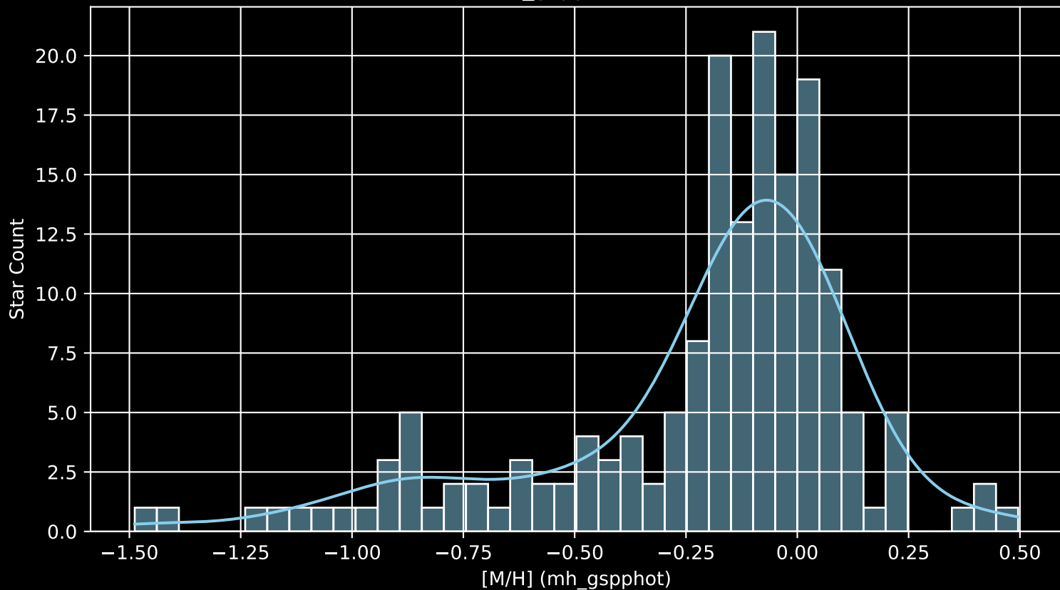
APOGEE DR17 Field: [235+00 [M/H] (mh_gspphot) (n= 169)
