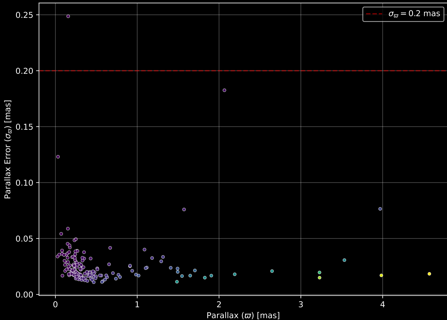
APOGEE DR17 Field: [235+00] Parallax Quality (n= 170)
