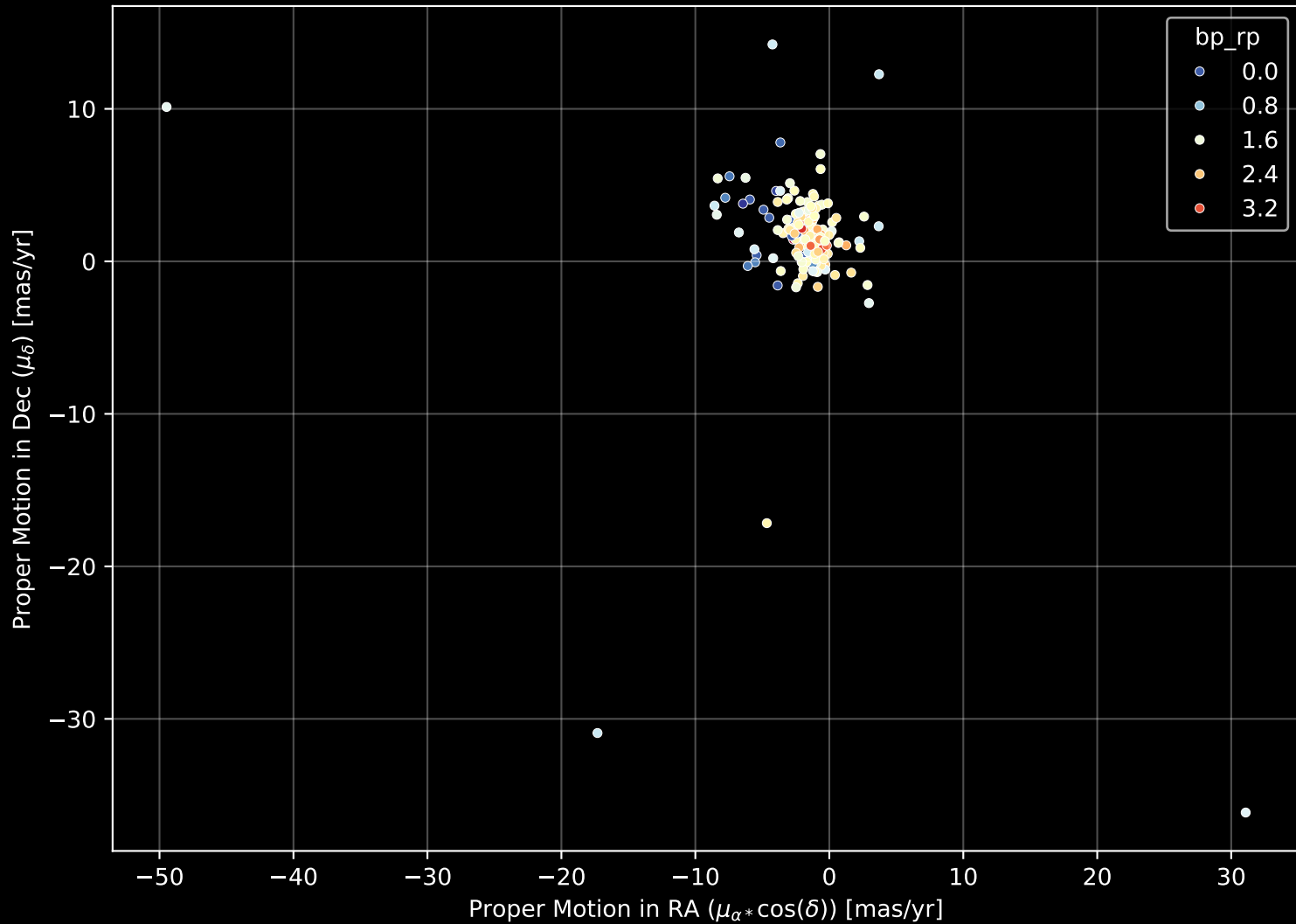
APOGEE DR17 Field: [235+00] Proper Motion Diagram (n= 170)
